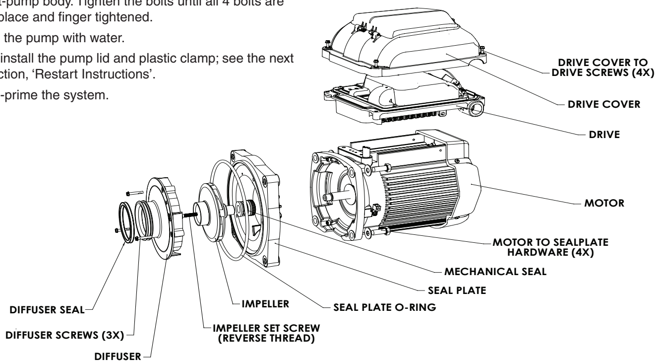
Motor Assembly
